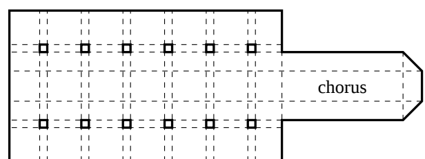
Fig. 1. Ground plan sketch of a typical Gothic church located in Germany. The dashed lines indicate the subdivision into rectangular and triangular block models.
