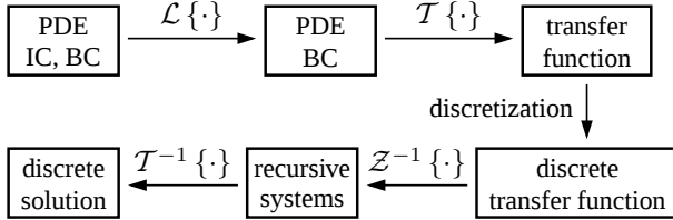
Fig. 2. General procedure of the FTM for solving initial boundary value problems in form of PDEs with initial- (IC) and boundary (BC) conditions. The transformations are explained in the remainder of this section.
