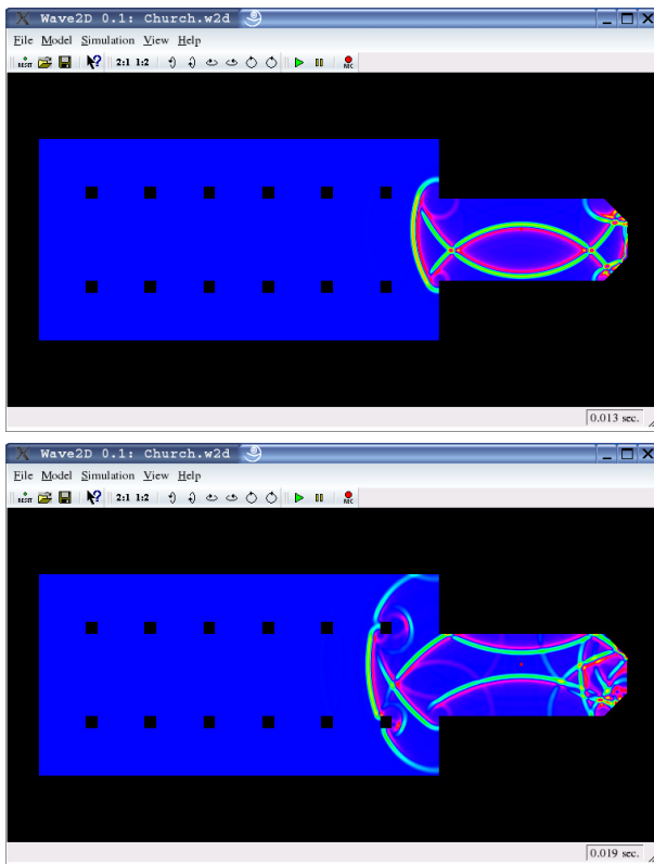
Fig. 4. Impulse propagation in a church simulated with “Wave2D”. Complete videos can be found in [6].
