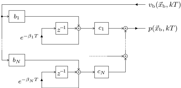
Fig. 3. Structure of the FTM implementation with N complex harmonics. Explicit values for the input weighting constants b_n and output weighting constants c_n can be found in [1].
